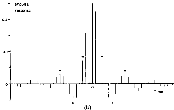
Fig. 2. Ideal filter responses for initial guess calculation. (a) Amplitude response. (b) Impulse response. Symbol \Delta indicates average delay time. Symmetrical conditions are imposed on samples designated by symbol *. Sampling frequency is 400 Hz.
