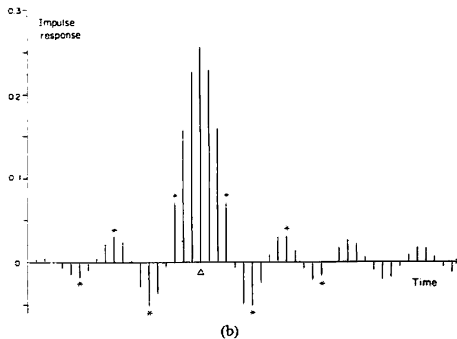
Fig. 2. Ideal filter responses for initial guess calculation. (a) Amplitude response. (b) Impulse response. Symbol \Delta indicates average delay time. Symmetrical conditions are imposed on samples designated by symbol *. Sampling frequency is 400 Hz.
