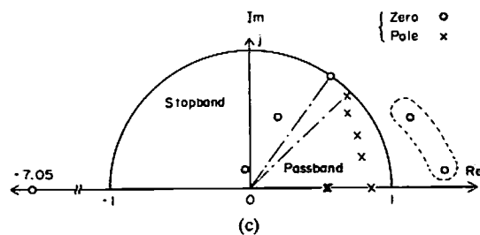
Fig. 3. Filter responses designed through proposed method with 11/11th-order transfer function, 20T average delay time and 400 Hz sampling frequency. (a) Amplitude response in decibels. (b) Impulse response. (c) Pole-zero locations.
