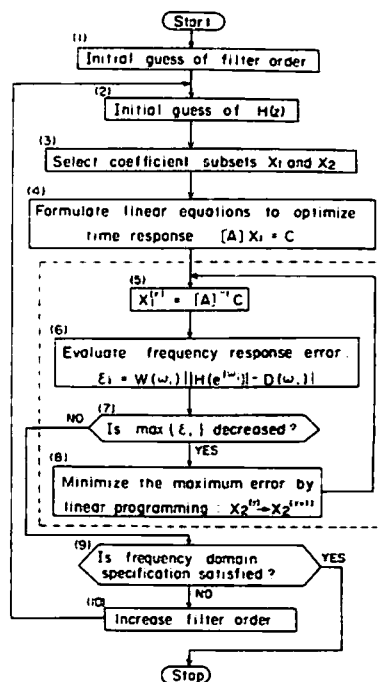
Fig. 1. Flowchart for simultaneous frequency- and time-domain approximation method.
