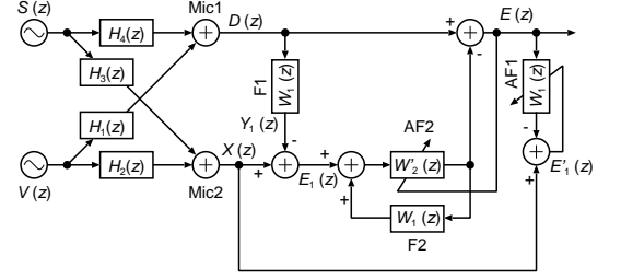
Fig. 7. Proposed Noise Canceller.
