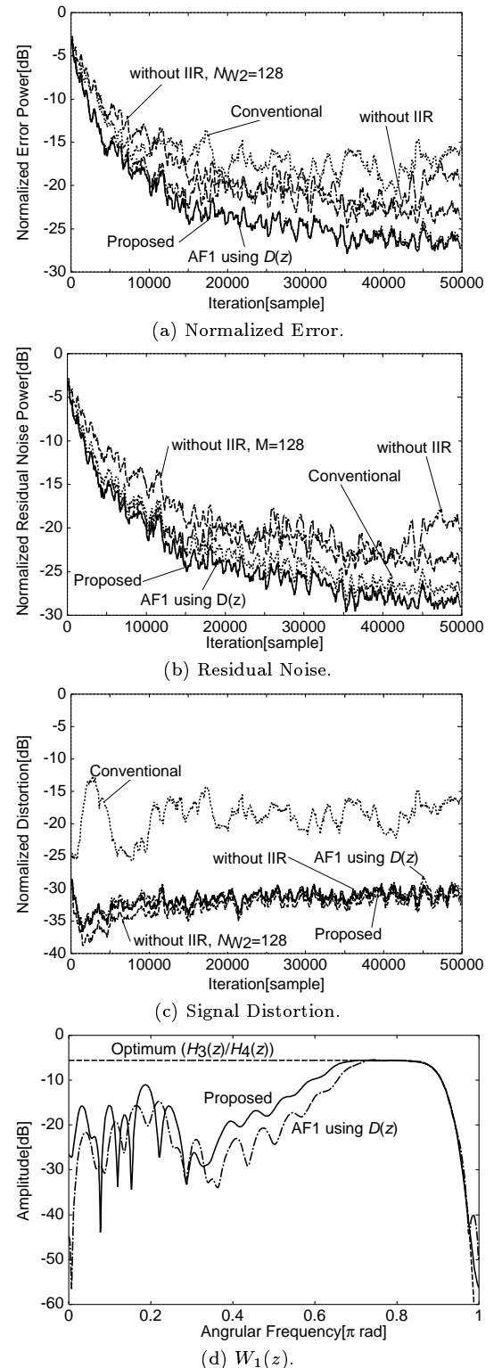
Fig. 11. Simulations for Colored Input.
