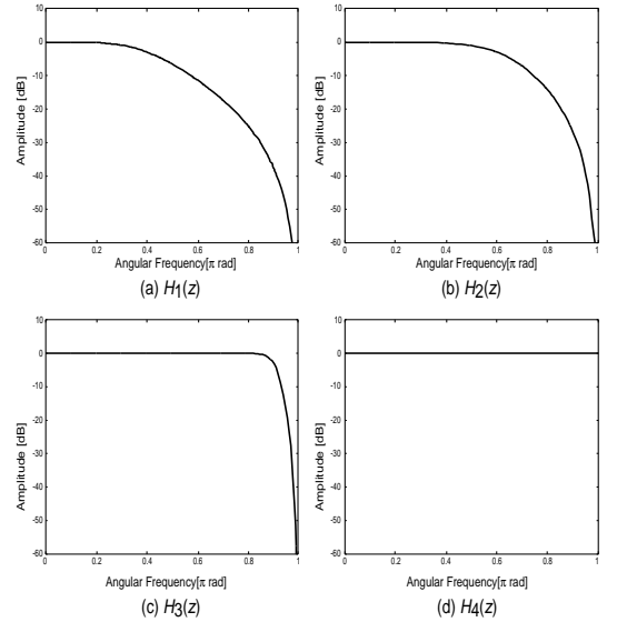
Fig. 9. Frequency Responses of Unknown Systems.
