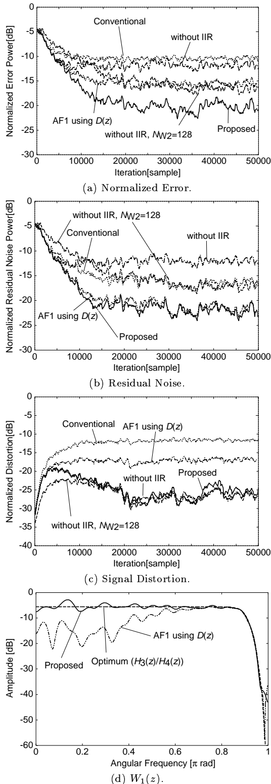
Fig. 10. Simulations for White-Noise Input.
