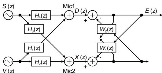
Fig. 2. Cross-Coupled Noise Canceller.
