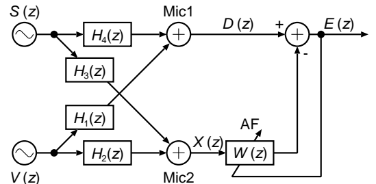
Fig. 1. Classical Noise Canceller in Presence of Crosstalk.
