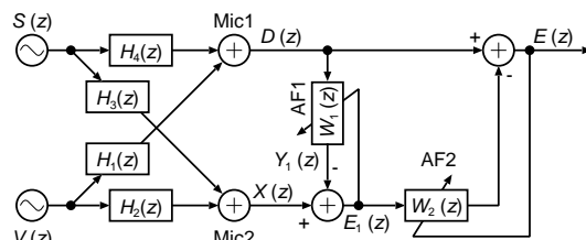
Fig. 5. Basic Block Diagram of Proposed Noise Canceller.
