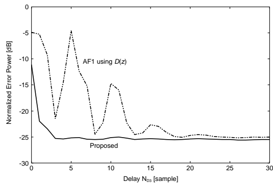
Fig. 12. Relation between N_{D3} and Error Power.
