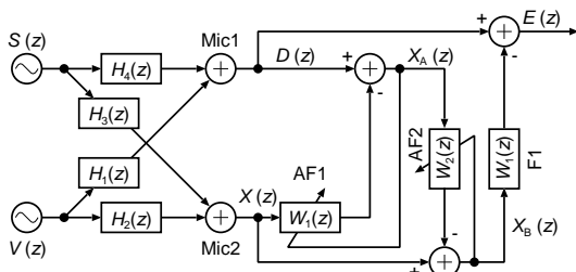
Fig. 3. Noise Canceller with Pre-Processing.
