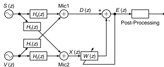
Fig. 4. Noise Canceller with Post-Processing.
