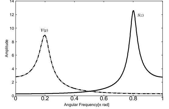
Fig. 8. AR Model for Colored Signals.
