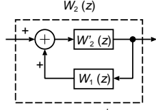
Fig. 6. Implementation of W_2^{opt}(z) by Recursive Filter.
