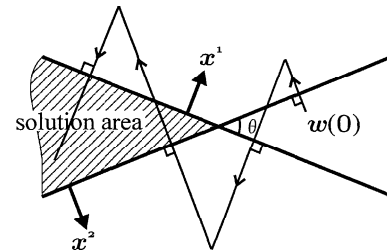
Fig. 2. Weights update process in 1-GLA.
